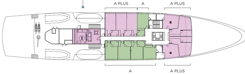
Upper Cabin Deck Astra
